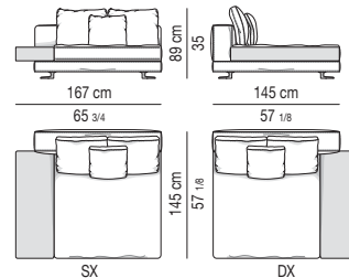
SOFÀ-ISOLA CHAISE LONGUE CON TOP CM 44X117 SOFÀ-CHAISE-LONGUE ISLE WITH TOP CM 44X117
