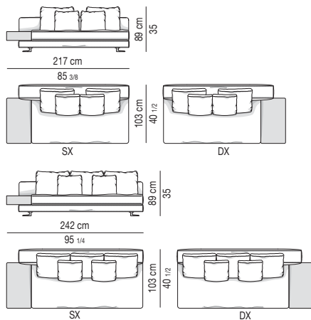
SOFÀ-MIX CON TOP CM 44X79 E 44X44 SOFÀ-MIX WITH TOP CM 44X79 AND 44X44
