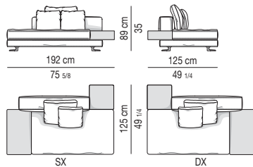
SOFÀ-MIX CON TOP CM 44X79 E 44X44 SOFÀ-MIX WITH TOP CM 44X79 AND 44X44
