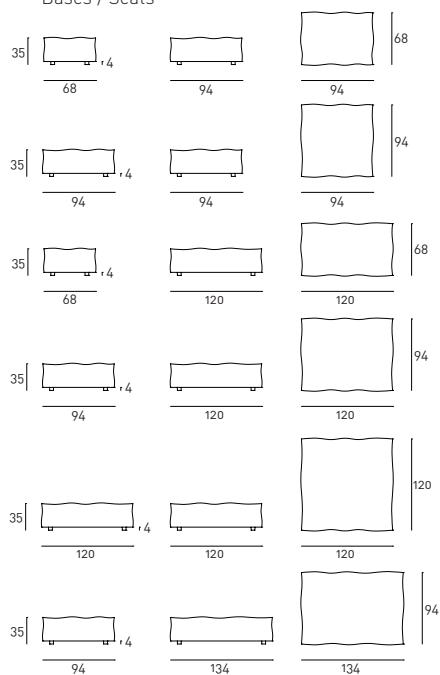
Bases / Seats
