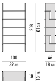
LIBRERIA CM 100X46 H208 - MOD. A BOOKCASE CM 100X46 H208 - MOD. A
