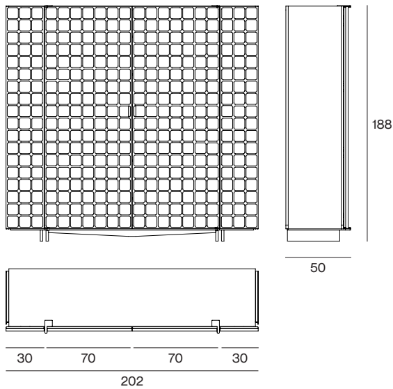
Checkmate Cabinet Cm 202x50x188h
