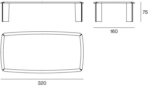
Grand Stand Cm 320x160x75h
