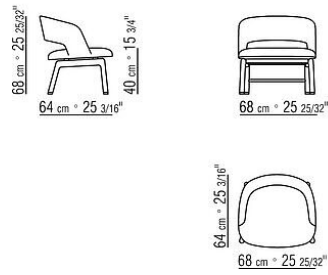
COD. 029844 ARMCHAIR W/ARMRESTS ALUMINUM BASE
