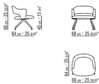
COD. 029847 ARMCHAIR W/ARMREST CANALETTO/OAK/WENGE FEET
